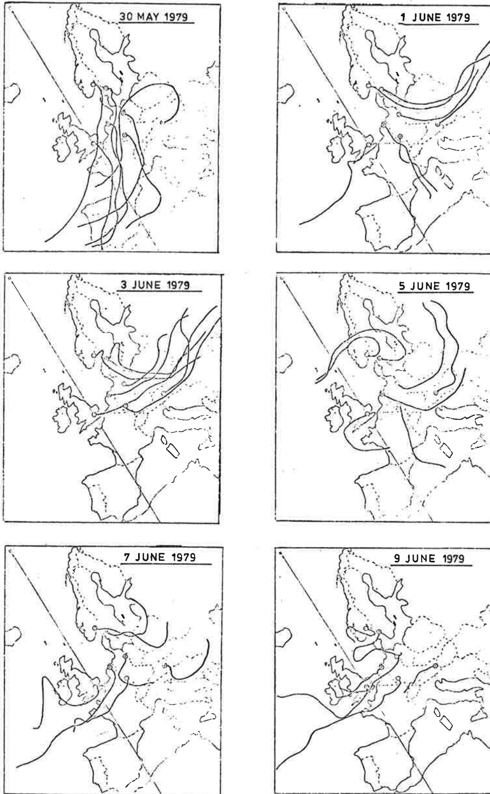
Figure 16: 96-h air trajectories at the 850 mb level, arriving at 12 GMT on every second day, 30 May-9 June 1979.
