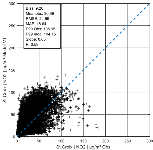
Figure A 66: Yearly value NO 2 in St. Croix, V1
