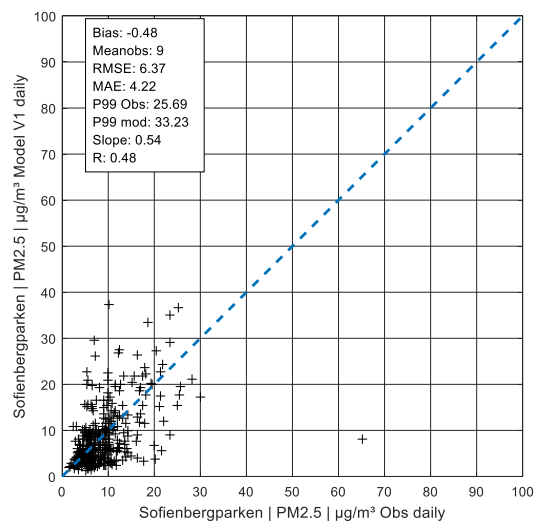
Figure A 159: Daily value PM 2.5 in Sofienbergparken, V1
