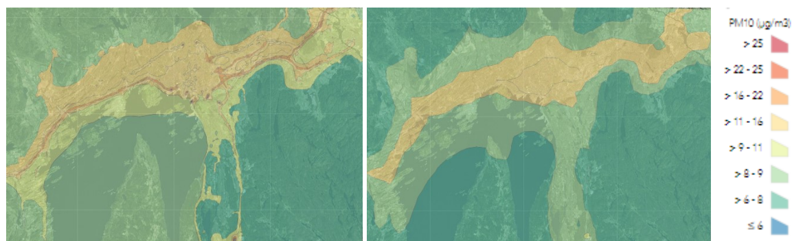
Figure 3.1.1. Modelled yearly mean of PM_{10} concentrations for 2015 in the Oslo-Bærum domain. The right panel shows results with standard 1x1km resolution. The left panel shows the same results taking into account sub-grid variability with a 100x100m resolution. Units:[ \mu g/m^3 ]
