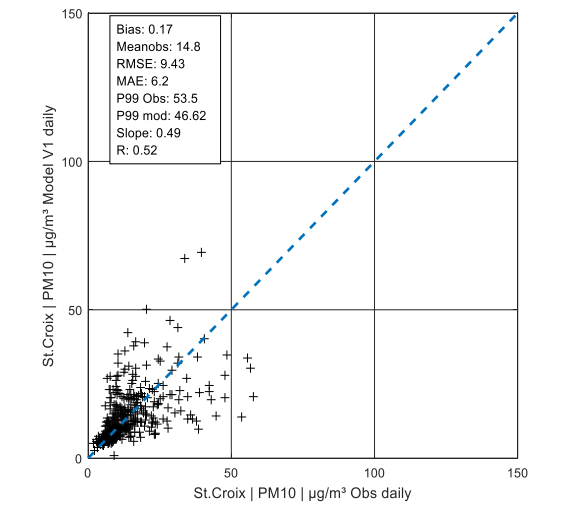
Figure A 72: Daily value PM 10 in St. Croix, V1
