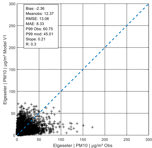
Figure A 202: Yearly value PM 10 in Elgeseter, V1
