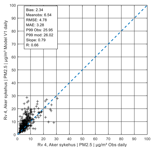
Figure A 153: Daily values PM 2.5 in Aker Sykehus, V1
