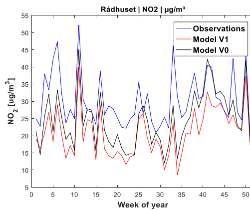
Figure A 8: Week of year NO 2 in Rådhuset
