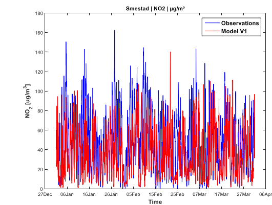
Figure A 105: Timesheet NO 2 in Smestad
