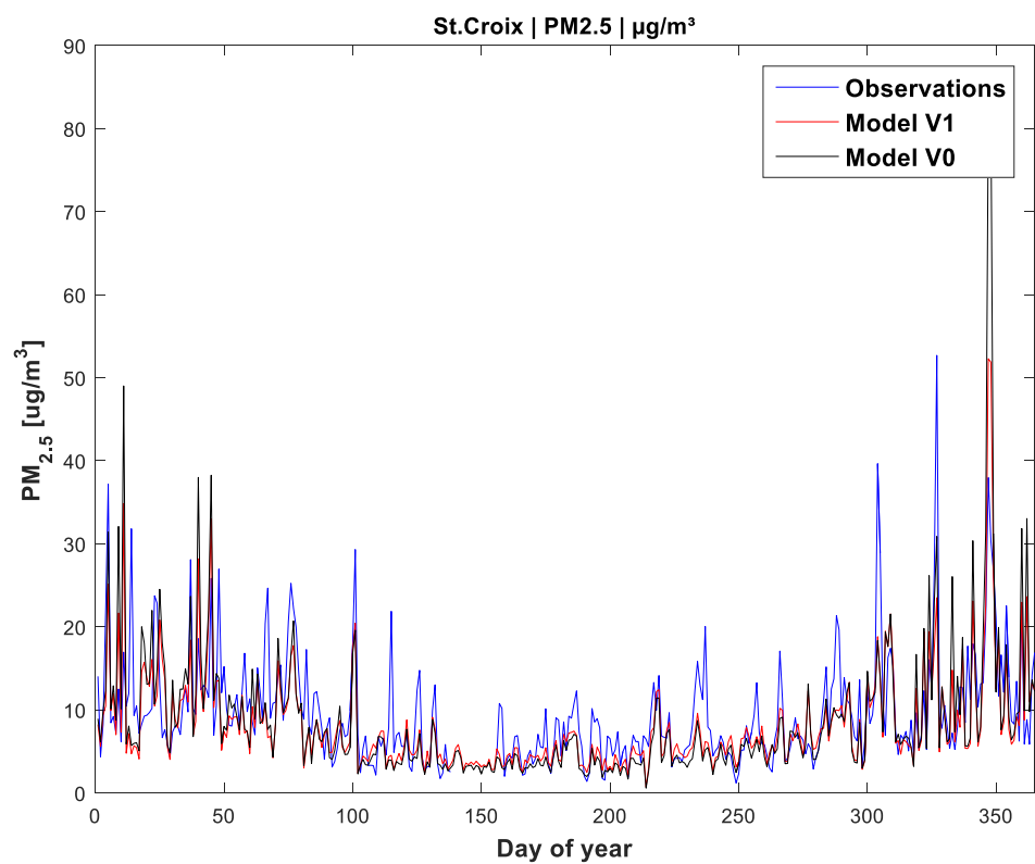
Figure A 79: Day of year PM 2.5 in St. Croix
