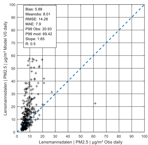
Figure A 59: Daily values PM 2.5 in Lensmannsdalen, V0
