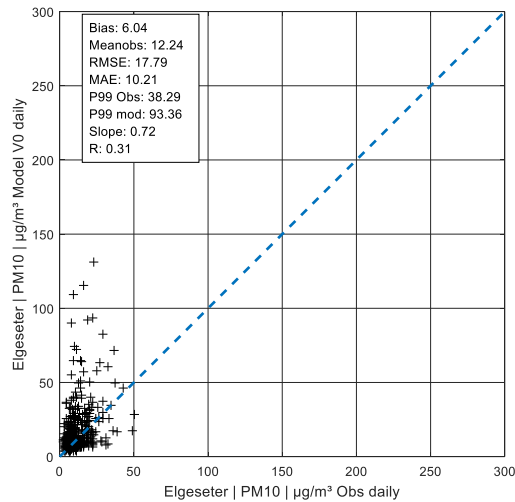
Figure A 205: Daily value PM 10 in Elgeseter, V0
