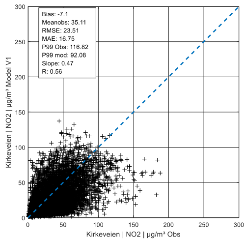
Figure A 95: Yearly value NO 2 in Kirkeveien, V1
