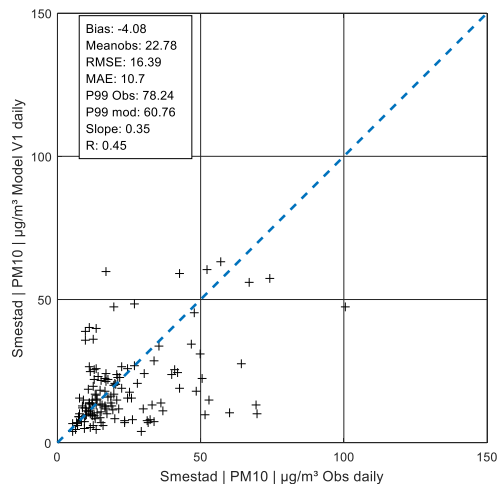
Figure A 128: Hourly values PM 10 in Smestad, V1 Figure A 129: Daily values PM 10 in Smestad, V1
