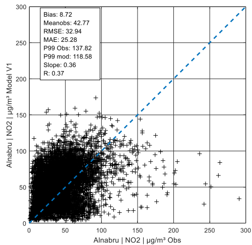
Figure A 83: Yearly value NO 2 in Alnabru, V1
