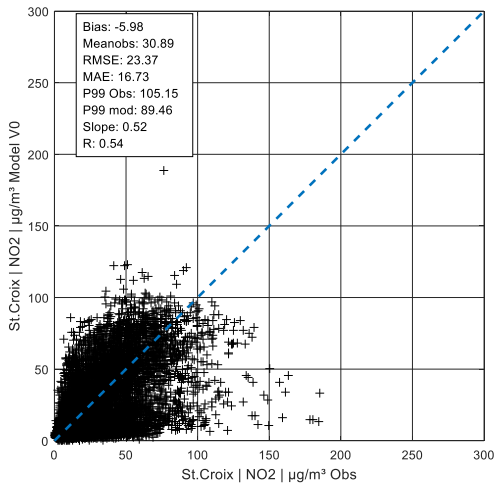
Figure A 67: Yearly value NO 2 in St. Croix, V0
