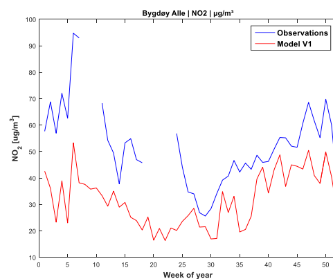
Figure A 88: Week of year NO 2 in Bygdøy, V1
