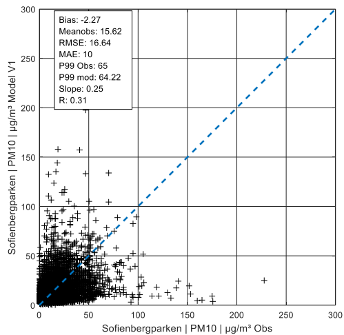
Figure A 131: Hourly values PM 10 in Sofienbergparken, V1
