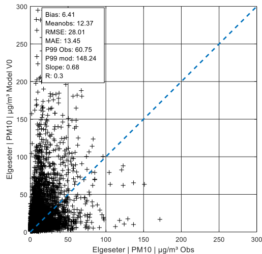
Figure A 203: Yearly value PM 10 in Elgeseter, V0
