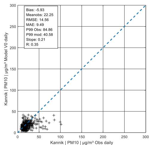
Figure A 172: Daily values PM 10 in Kannik, V0
