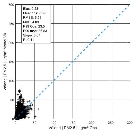
Figure A 185: Hourly values PM 2.5 in Våland, V0
