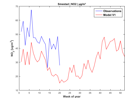
Figure A 106: Week of year NO 2 in Smestad
