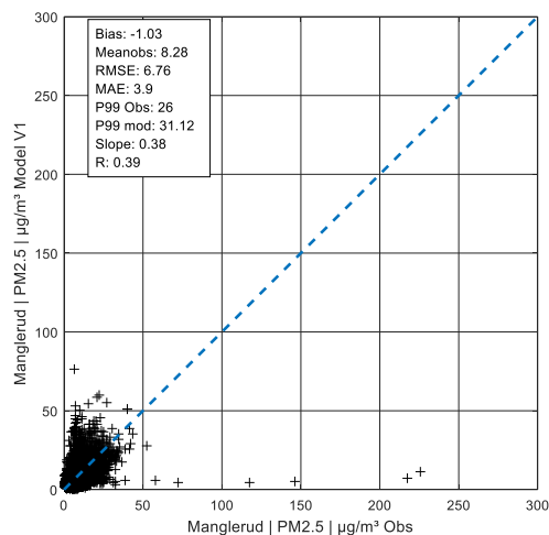
Figure A 149: Hourly values PM 2.5 in Manglerud, V1
