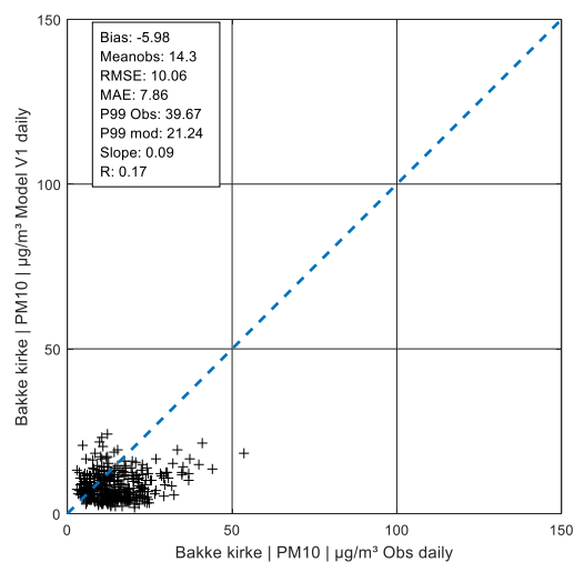
Figure A 199: Daily values PM 10 in Bakke kirke, V1
