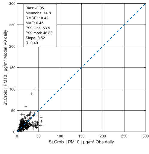
Figure A 73: Daily value PM 10 in St. Croix, V0
