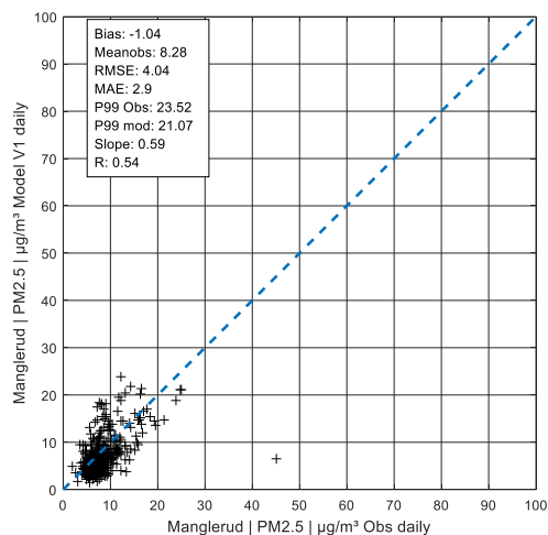
Figure A 150: Daily values PM 2.5 in Manglerud, V1
