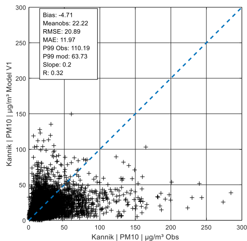
Figure A 169: Hourly values PM 10 in Kannik, V1
