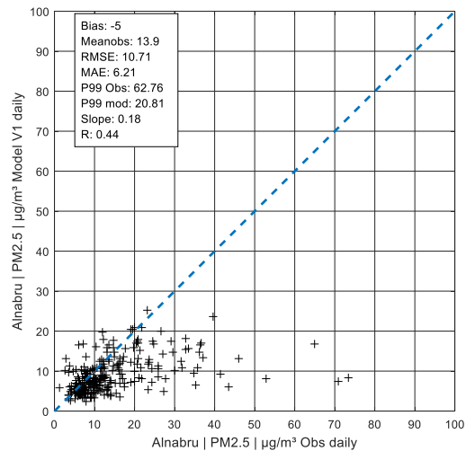
Figure A 137: Hourly values PM 2.5 in Alnabru, V1 Figure A 138: Daily values PM 2.5 in Alnabru, V1
