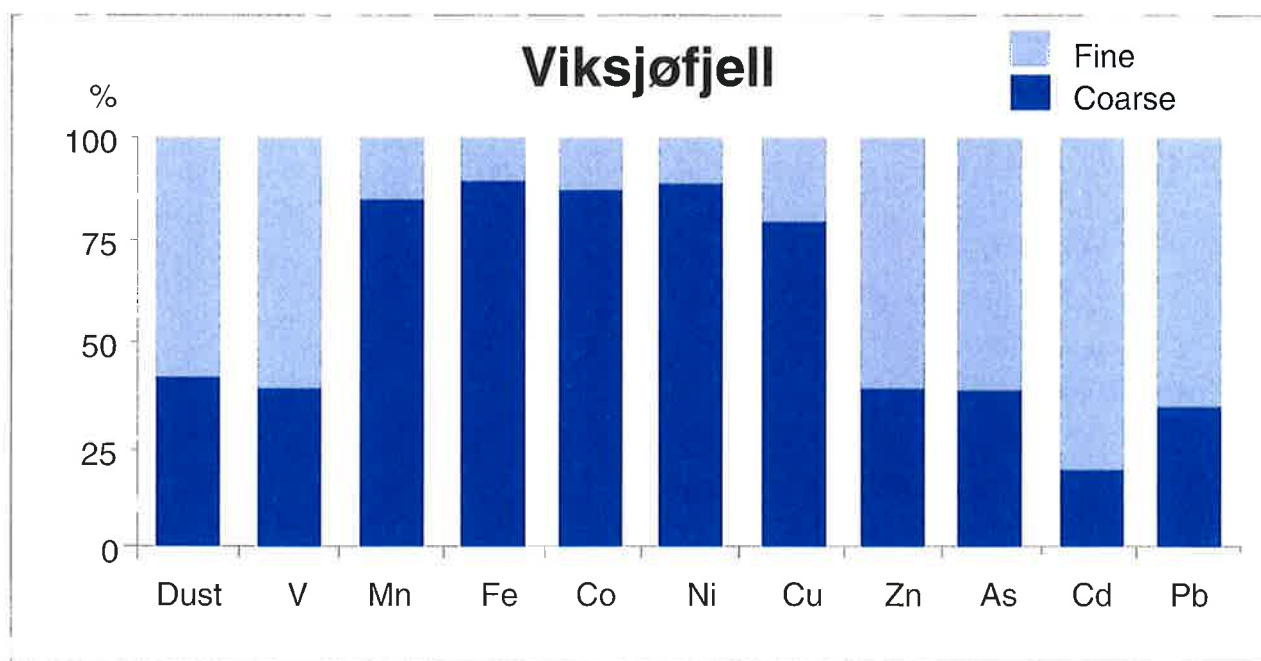
Figure 6: Distribution of elements in fine (<2.5 μm) and coarse fraction (2.5-10 μm) and suspended dust at Viksjøfjell (1992-93). A similar pattern can be seen at Maajavri and Svanvik.
