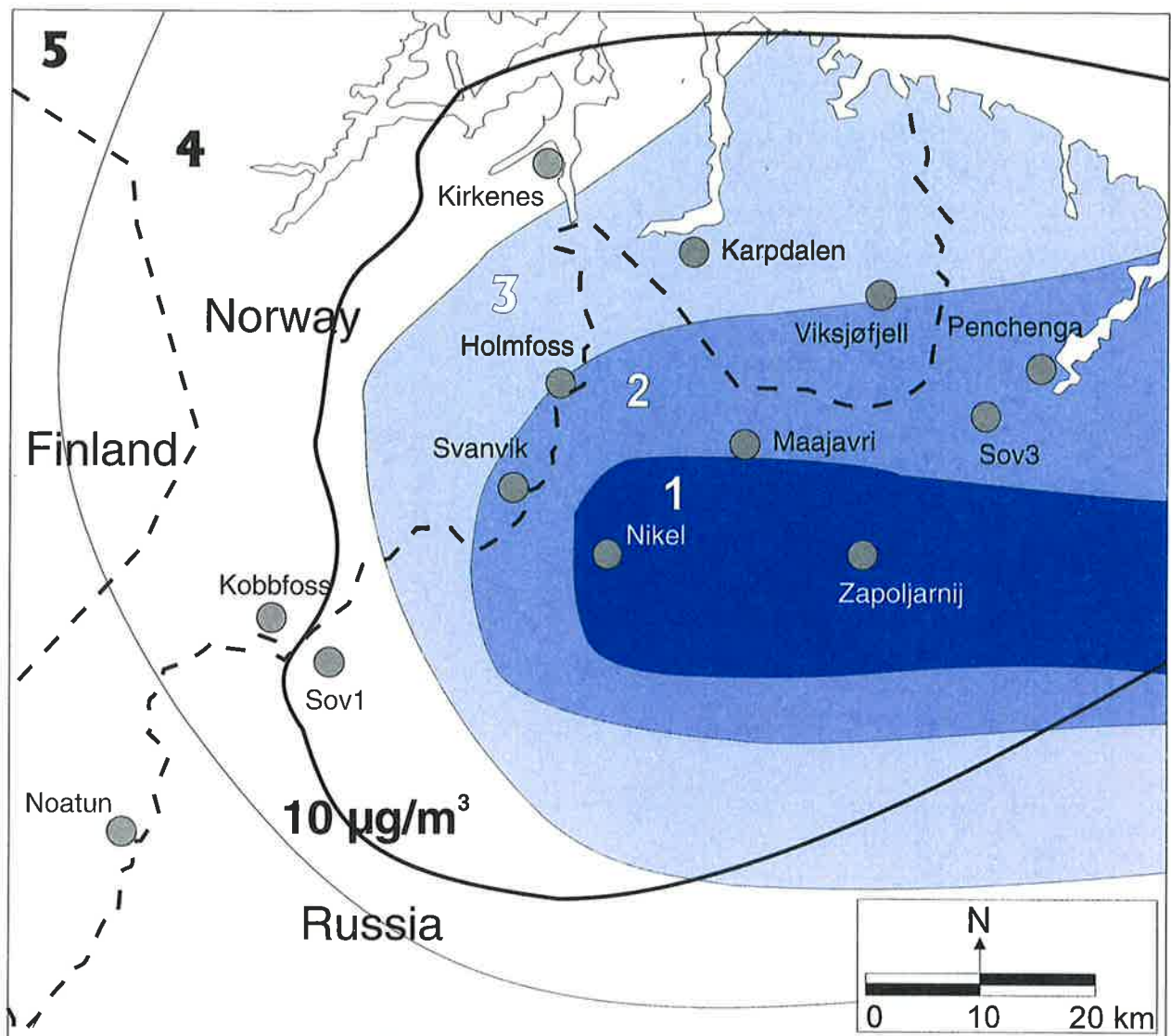
Figure 9: Different damage zones in the border areas of Norway and Russia.
