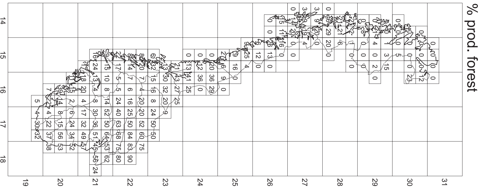
Figure 1.2: Percent productive forest used in estimating dry deposition.
